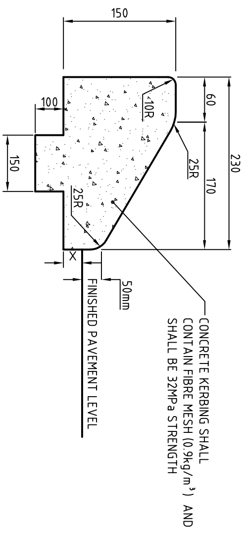
SEMI MOUNTABLE KERB DETAIL (MRD TYPE)
